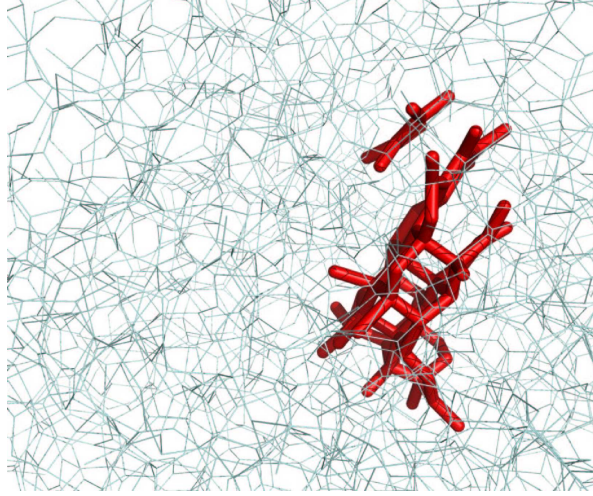
Figure 6.1.: Typical snapshot of a small crystalline cluster of \sim 75 particles obtained at 30 GPa and 3750 K (state point B ), surrounded by mainly three-fold coordinated liquid particles. The figure shows both three/four-fold coordinated particles (upper half). The grey lines surrounding the cluster indicate bonds between liquid carbon atoms.
