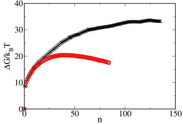
Figure 5.3.: Free-energy barriers calculated with Umbrella Sampling at T^*=1 and P^*=15 in an 8000 particles system. The CsCl clusters have lower free energy, but unless unphysical Monte Carlo moves are used in the sampling, the system remains kinetically trapped in a disordered fcc route of higher free energy.
