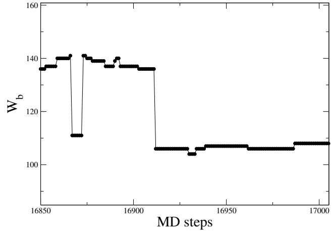
Figure 8.3.: Fluctuations of the order parameter as a function of MD time steps for a generic FFS-interface at T^* = 0.855 and P^* = 0.026 . The “nonphysical” effect due to anomalous conformation of the bubble, made of two sub-bubbles attached by a narrow non-liquid-like volume, results in a jump of W_b .
