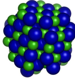
Figure 9.2.: Average shape of a NaCl crystallite consisting of 140 solid-like particles.
