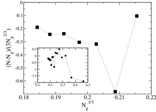
Figure 9.C.5.: Estimation of a at the equi-enthalpy dividing surface for different cluster sizes ranging from 100 to 160 particles. The inset shows that, for clusters smaller than 100 particles, the value of a is quite noisy. In the inset, the x and the y axes represent the same variables.
