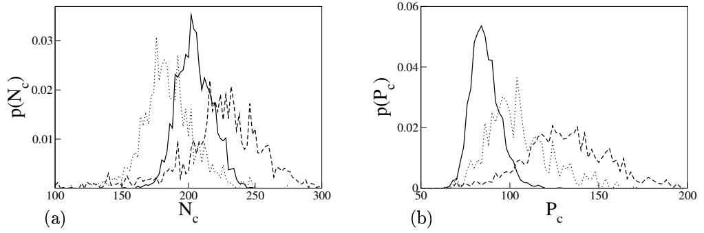
Figure 10.6.: Distributions of the biggest cluster sizes N_c (panel (a)) and perimeters P_c of the biggest cluster (panel(b)) for points in the TSE, for shear rates \dot{\gamma} = 0.0 (continuous line), \dot{\gamma} = 0.06 (dotted line) and \dot{\gamma} = 0.12 (dashed line).
