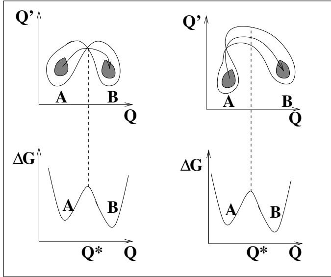
Figure 2.5.: At the top, the phase space is projected onto two order parameters Q and Q' , A and B being the basins of attractions; at the bottom, the free energy as a function of Q . On the left-hand side, Q is a good reaction coordinate, differently from the right side (figure copied from ref. [35]).
