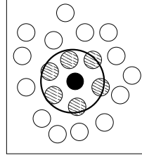
Figure 2.A.1.: The two-dimensional sketch indicates particle i (black at the centre) surrounded by its neighbours j (striped particles) within the cut-off radius r_c . The remaining particles (white) are not i 's neighbours.
